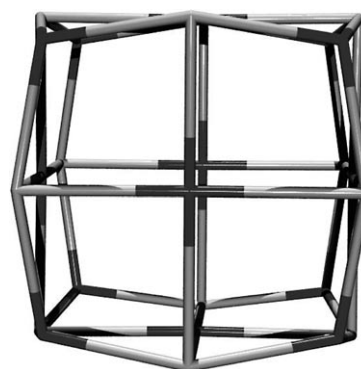
Figure 2. Wireframe representation of the central [\text{Ti}_{12}\text{O}_{14}]^{20+} core. Titanium and oxygen atoms in light and dark grey, respectively.
